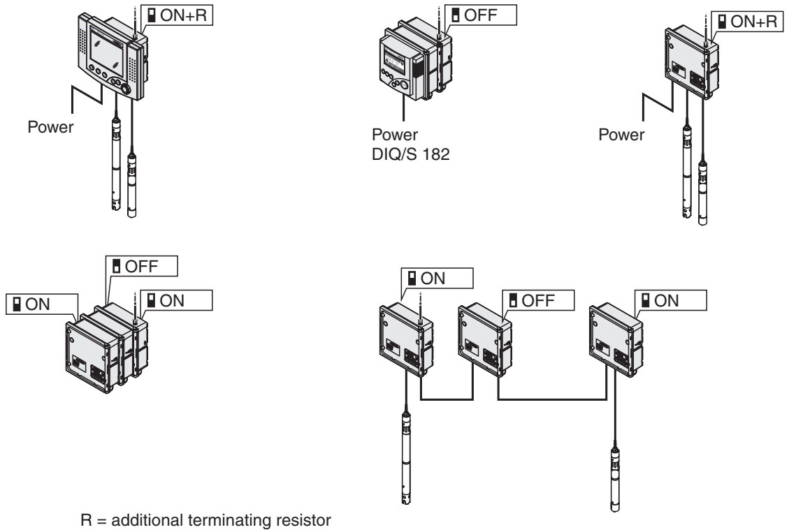
Fig. 3-5 Terminator switches and terminating resistors
