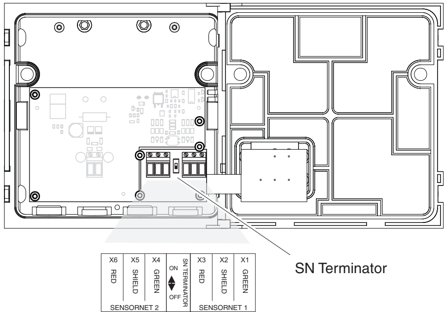
Fig. 3-3 Terminator switch
